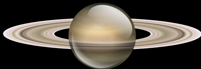
Planet Saturn
