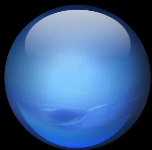
Planet Neptune
