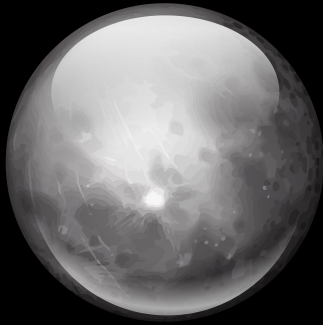
Planet Mercury
